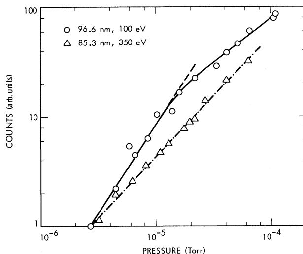
FIG. 3. Pressure linearity tests for two spectral features indicated in Table I. These features are predominantly the (2,0) Werner band at 96.6 nm and the D(2,0) band at 85.3 nm.
