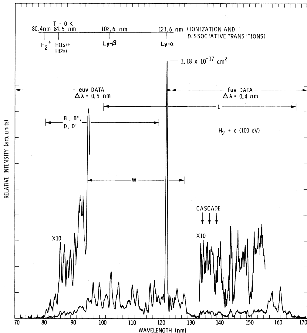
FIG. 4. Calibrated laboratory spectrum of H_2 at 100-eV electron impact energy. Arrows indicate wavelength regions of strong cascading emission. euv data were measured in this work and the fuv data were analyzed in a previous paper. 5 Spectra were joined at about 123 nm. Wavelength resolution was 0.5 nm for the euv data and was 0.4 nm for the fuv data. Background pressures in the chamber were 8 \times 10^{-6} Torr for the euv data and 2 \times 10^{-5} Torr for the fuv data.
