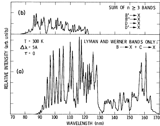
FIG. 11. (a) A theoretical model of the Lyman and Werner bands only at 0.5-nm resolution. \tau is the optical depth and T is the temperature. (b) A theoretical model of the B'-X, B''-X, D-X, and D'-X band systems at 0.5-nm resolution.
