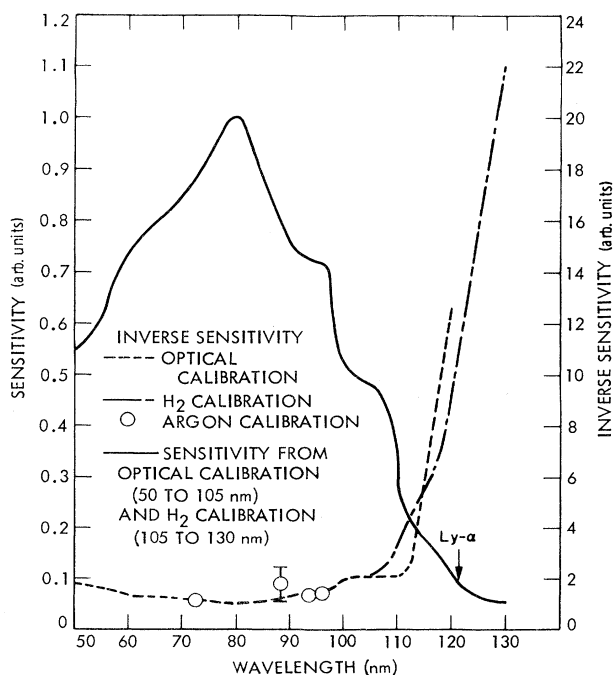
FIG. 2. Instrumental sensitivity and inverse sensitivity are shown as a function of wavelength as determined by three separate calibration techniques. The A\ II multiplets are at 72.5, 92.0, and 93.2 nm. The two A\ I multiplets near 87 nm lead to a calibration value that is uncertain by 30% (error bars indicated) due to radiation trapping effects.
