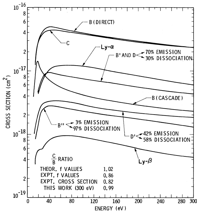
FIG. 7. A complete set of electronic cross sections for H_2 from electron impact based on Table II for the molecular transitions, Table IV for the Ly- \beta transition and on the work of Mumma and Zipf (Ref. 19) for Ly- \alpha . Included in the graph are important C/B ratios as discussed in Ajello et al. (Ref. 5) in Table I and the discussion section of that reference. Note the B' and D cross-section curves are shown as the same.
