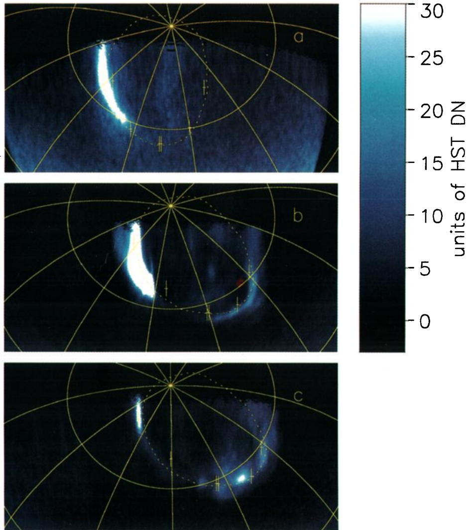
Plate 4. Jupiter's dawn auroral storms from three HST imaging observations, projected to a uniform point of view from above the central meridian and +60^\circ latitude. Details of the three images are listed in Table 2. The dashed line in each panel indicates the WFPC 2 reference oval at the midpoint of the exposure, and the hatch marks overplotted on each reference oval indicate the locations of magnetic local dawn, 0300 hours, noon (double hatch marks), 1500 hours, and dusk. The dawn storm emissions can be seen to be close to the reference oval on each occasion, with a significant spreading in longitude which in each case also covers magnetic local dawn. In each case the bright emission extends to the limb, and its extent onto the nightside is unknown.
