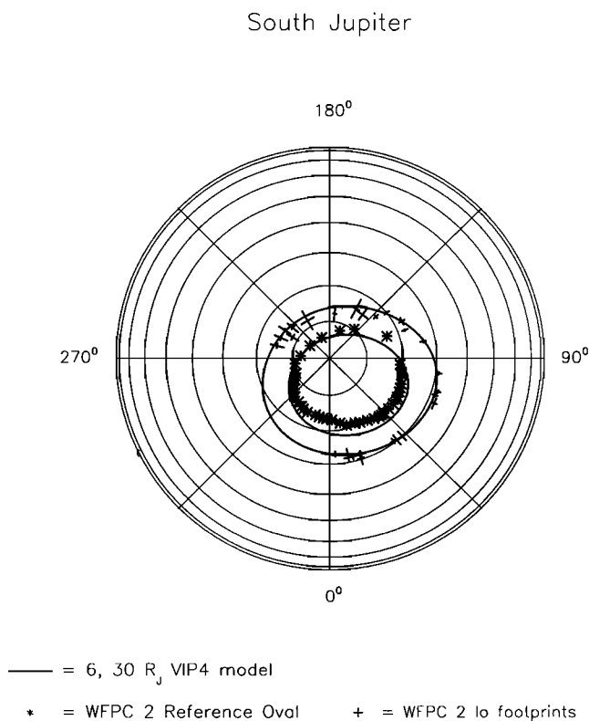
Figure 2b. South pole projections showing the "WFCP 2" reference auroral ovals (stars) from March 1995 overplotted with the locations of the 6 and 30 R_J ovals in the VIP4 planetary magnetic field model (solid lines). The regions where few points are plotted indicate regions appearing near the limb, where the model ovals are more uncertain. Crosses indicate the location of Io footprint emissions, with the lengths of the lines indicating measurement uncertainties.
