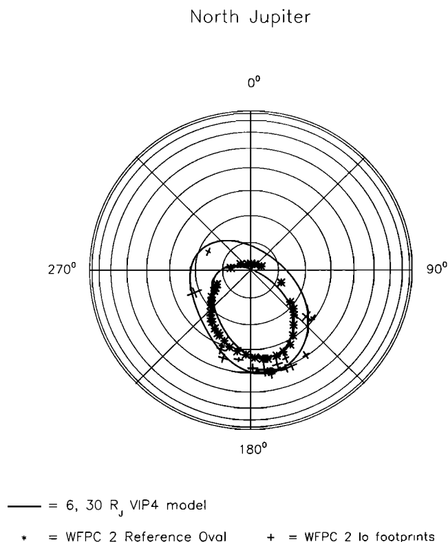
Figure 2a. North pole projections showing the "WFCP 2" reference auroral ovals (stars) from March 1995 overplotted with the locations of the 6 and 30 R_J ovals in the VIP4 planetary magnetic field model (solid lines). The regions where few points are plotted indicate regions appearing near the limb, where the model ovals are more uncertain. Crosses indicate the location of Io footprint emissions, with the lengths of the lines indicating measurement uncertainties.
