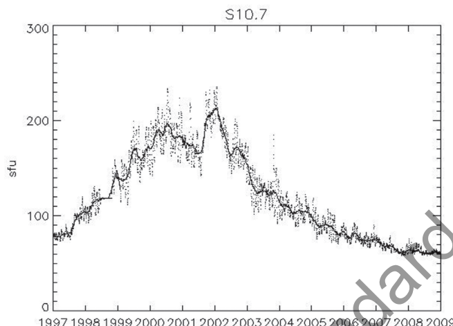
Figure B.1 — S_{10.7}(\text{v4.0}) daily and 81-day smoothed values for use by the JB2008 model from January 1, 1997 to January 1, 2009
