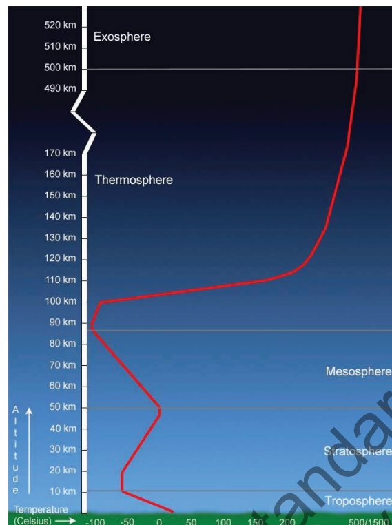
Figure A.1 — Temperature profile of the Earth's atmosphere
