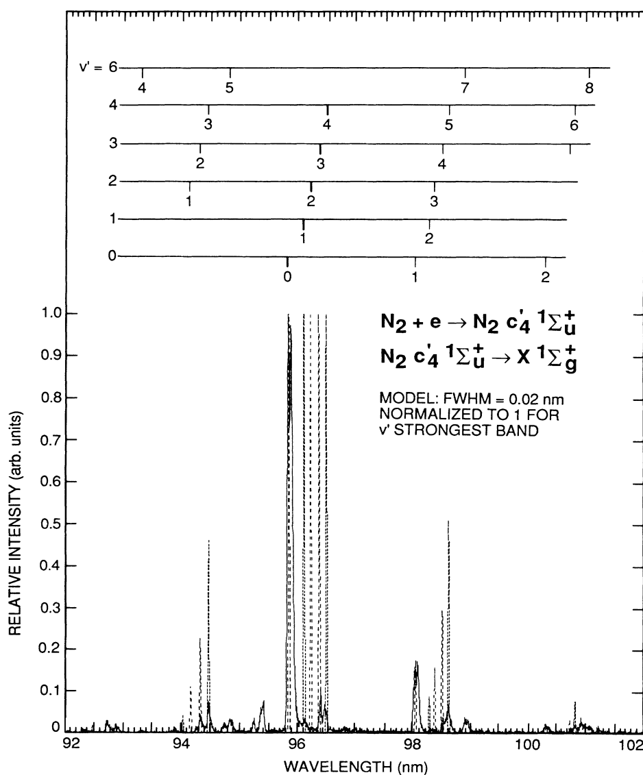
FIG. 11. Calibrated optically thin spectrum of \text{N}_2 from Fig. 9 overplotted with model of c'_4 1\Sigma_u^+ \rightarrow X 1\Sigma_g^+ band system from Fig. 8 for v'=0, 1, 2, 3, 4 progressions normalized to peak value in each progression. The model data were normalized to unity for each progression separately to bring strongest features on scale.
