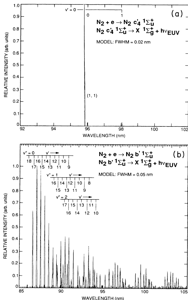
FIG. 8. (a) Synthetic direct excitation spectrum of c'_4 \ 1\Sigma_u^+ \rightarrow X \ 1\Sigma_g^+ bands based on diabatic potential curves in Fig. 7 without rotational structure. The molecular constants are taken from Huber and Herzberg (Ref. 11). The synthetic spectrum is convolved with a 0.02-nm triangular instrumental band pass. (b) Synthetic direct excitation spectrum of b' \ 1\Sigma_u^+ \rightarrow X \ 1\Sigma_g^+ bands with a 0.05-nm band pass. The band heads for the (v',0) transition are from Lofthus and Krupenie (Ref. 12). The band origins from the nonresonance transitions are from Roncin, Launay, and Yoshino (Ref. 17). The calculated band origins are not sufficiently accurate using molecular constants of Huber and Herzberg (Ref. 11) to compare to the data for high v' .
