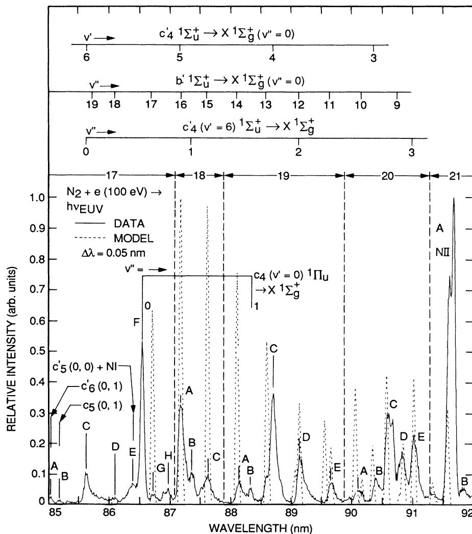
FIG. 13. Calibrated optically thin spectrum of N_2 from 85 to 92 nm produced by electron impact at 100 eV overplotted with synthetic spectrum of Fig. 8 for the b'1\Sigma_u^+ \rightarrow X1\Sigma_g^+ BH-II band system. Data and model are at 0.05-nm resolution.
