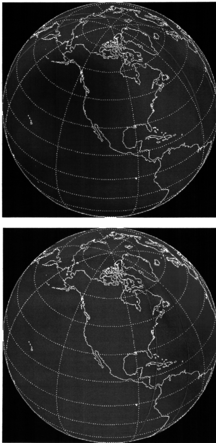
Plate 1. Top panel shows MSIS atmosphere on July 25, 1999 using E_{10.7} and a_p under quiet solar and geomagnetic conditions. The bottom panel shows the MSIS atmosphere on July 30, 1999, using E_{10.7} and a_p under perturbed solar and geomagnetic conditions. Color variations are relative with red indicating denser atmosphere and blue-green indicating less dense atmosphere.
