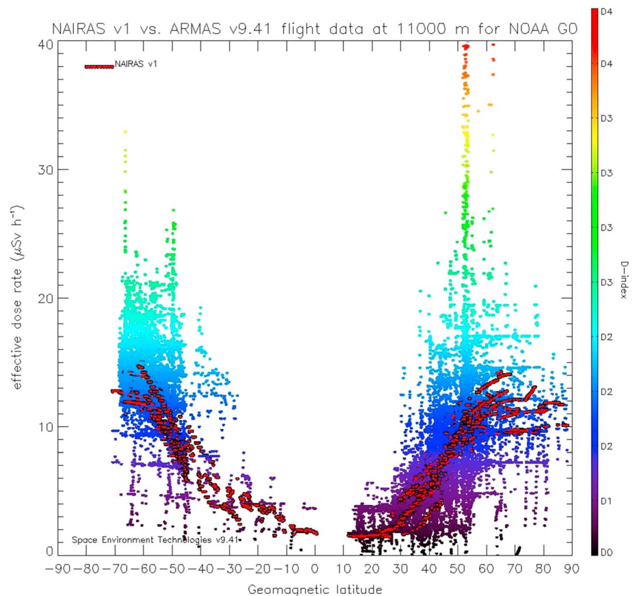
Figure 5. ARMAS derived effective dose rate (colored dots) compared with NAIRAS (red dots circled in black) for NOAA G0 geomagnetic conditions at 11 km for all geomagnetic latitudes. ARMAS = Automated Radiation Measurements for Aerospace Safety; NAIRAS = Nowcast of Atmospheric Ionizing Radiation for Aviation Safety; NOAA = National Oceanic and Atmospheric Administration.
