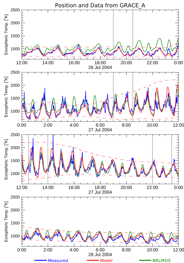
Figure 7. Example of exospheric temperatures along the GRACE A orbit, from 12 UT on 26 July to 12 UT on 28 July 2004. Solid red lines show the temperatures from the EXEMPLAR model evaluated along the orbit, while the dashed red lines show the smallest and largest values on the global grid at the same times. Blue lines show the measured values, and green lines show the temperatures in the MSIS model.
